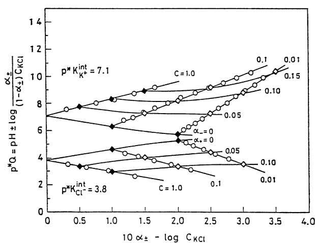
Fig. 5. Double extrapolation plot for determination of \text{p}^*K_{\text{K}^+}^{\text{int}} and \text{p}^*K_{\text{Cl}^-}^{\text{int}} showing the variation of surface complexation quotients, \text{p}^*Q , for positive and negative sites on maghemite ( \gamma\text{-Fe}_2\text{O}_3 ) in aqueous dispersion at 25 °C, with fractional ionization and KCl electrolyte concentration.
