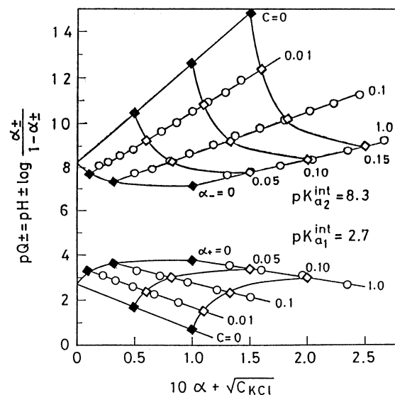
Fig. 3. Double extrapolation plot for determination of \text{p}K_{a1}^{\text{int}} and \text{p}K_{a2}^{\text{int}} showing the variation of surface acidity quotients, \text{p}Q_a , for dissociation of positive and negative sites on maghemite ( \gamma - \text{Fe}_2\text{O}_3 ) in aqueous dispersion at 25 °C, with fractional ionization and KCl electrolyte concentration.
