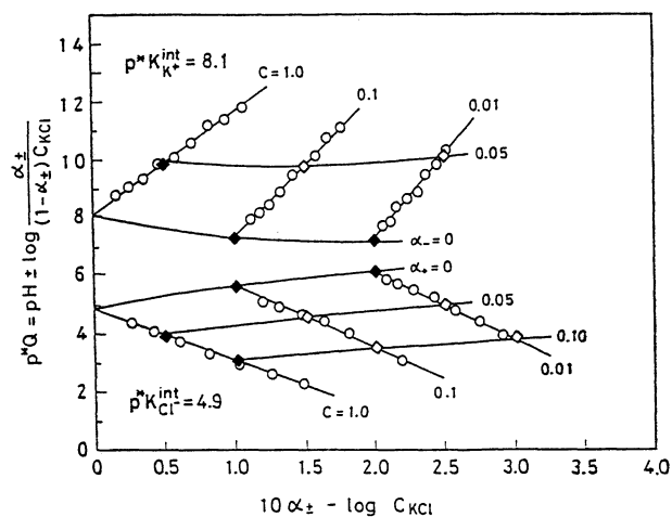
Fig. 6. Double extrapolation plot for determination of p^*K_{\text{K}^+}^{\text{int}} and p^*K_{\text{Cl}^-}^{\text{int}} showing the variation of surface complexation quotients, p^*Q , for positive and negative sites on hematite ( \alpha\text{-Fe}_2\text{O}_3 ) in aqueous dispersion at 25°C, with fractional ionization and KCl electrolyte concentration.
