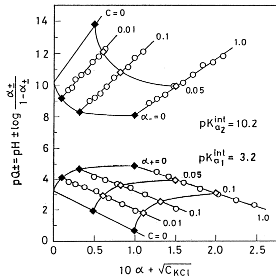
Fig. 4. Double extrapolation plot for determination of \text{p}K_{a1}^{\text{int}} and \text{p}K_{a2}^{\text{int}} showing the variation of surface acidity quotients, \text{p}Q_a , for dissociation of positive and negative sites on hematite ( \alpha - \text{Fe}_2\text{O}_3 ) in aqueous dispersion at 25 °C, with fractional ionization and KCl electrolyte concentration.
